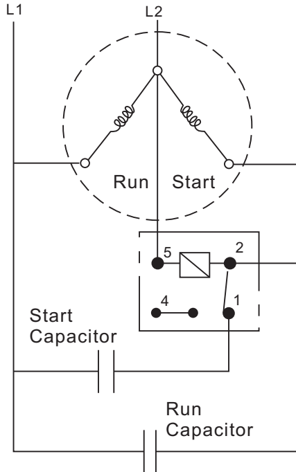
Wiring Diagram
